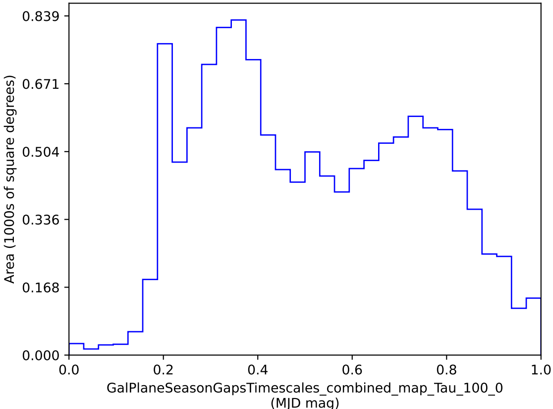
weather_cloudso10v3.4_10yrs : GalPlaneSeasonGapsTimescales_combined_map_Tau_100_0
