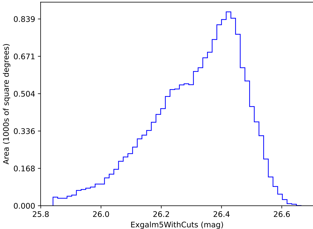
weather_cloudso10v3.4_10yrs i band non-DD year 9: ExgalM5WithCuts
