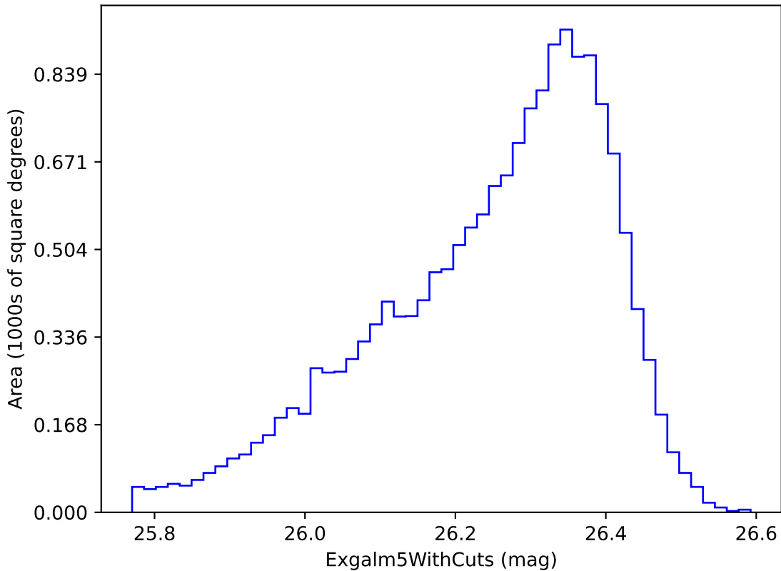
weather_cloudso10v3.4_10yrs i band non-DD year 8: ExgalM5WithCuts
