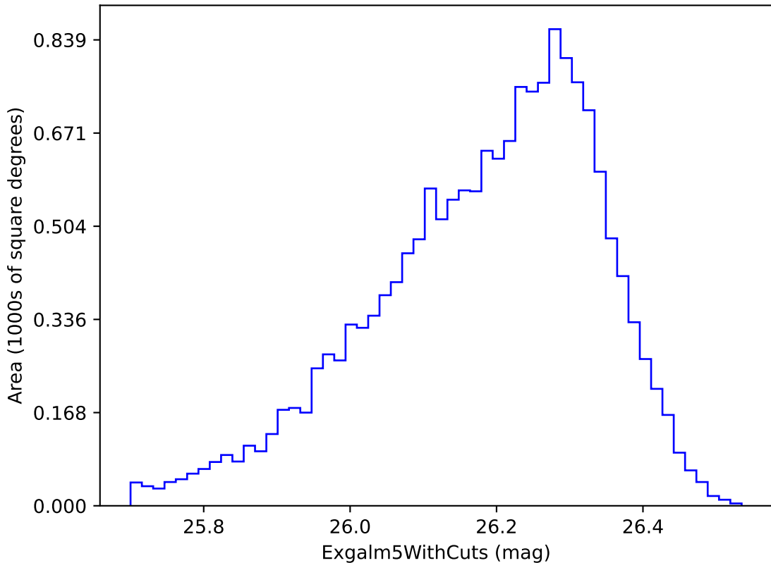
weather_cloudso10v3.4_10yrs i band non-DD year 7: Exgalml5WithCuts
