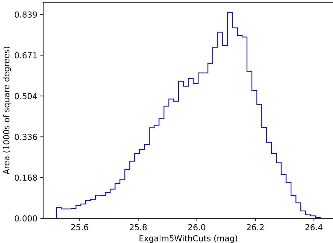
weather_cloudso10v3.4_10yrs i band non-DD year 5: ExgalM5WithCuts
