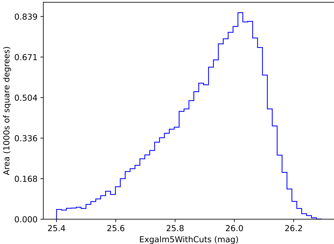
weather_cloudso10v3.4_10yrs i band non-DD year 4: ExgalM5WithCuts
