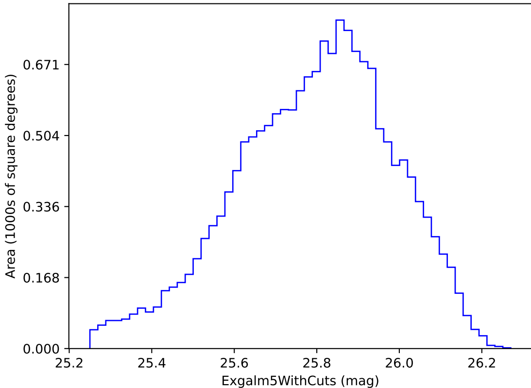
weather_cloudso10v3.4_10yrs i band non-DD year 3: ExgalM5WithCuts
