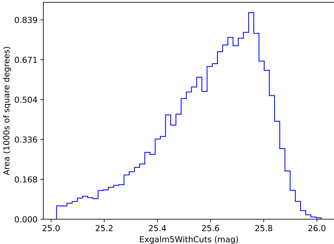
weather_cloudso10v3.4_10yrs i band non-DD year 2: ExgalM5WithCuts
