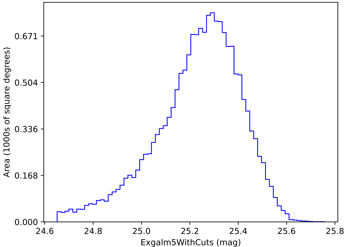
weather_cloudso10v3.4_10yrs i band non-DD year 1: ExgalM5WithCuts
