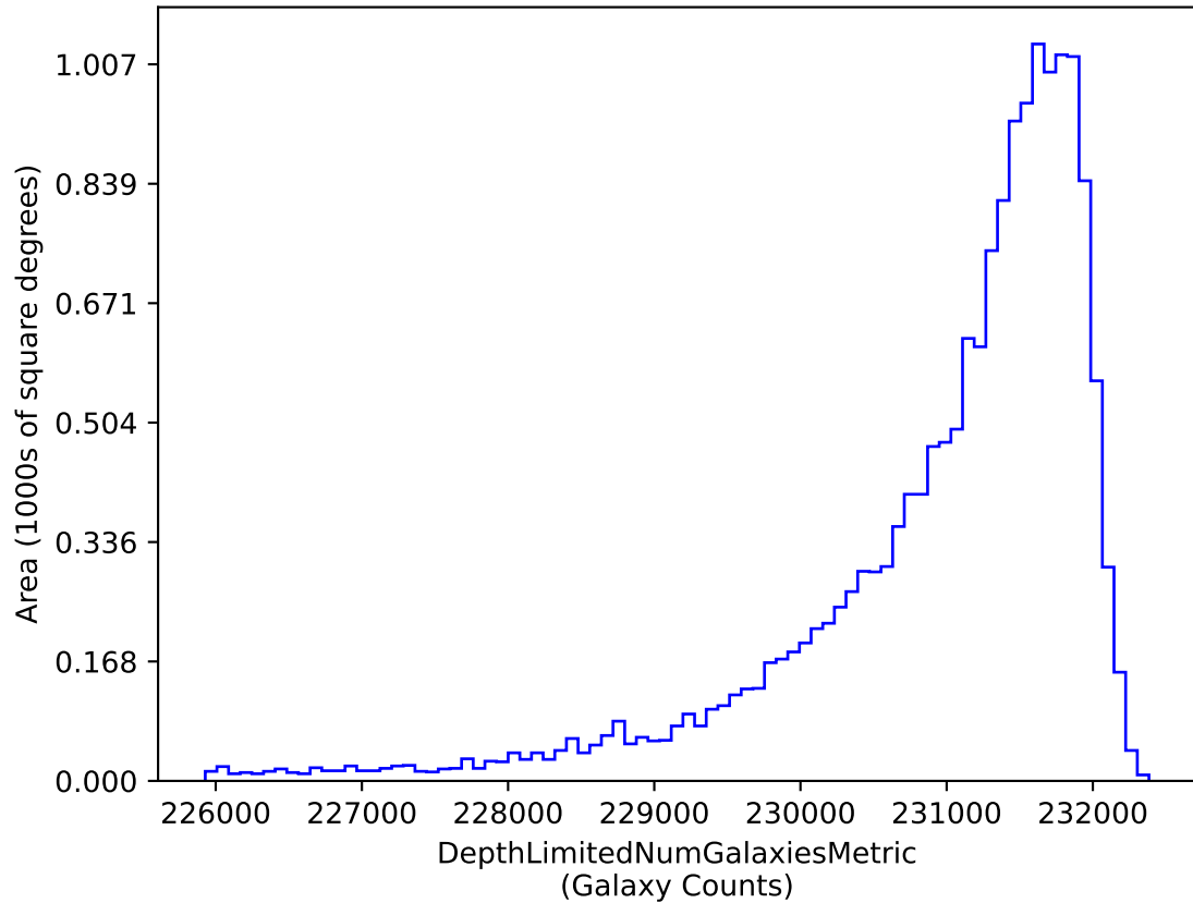
weather_cloudso10v3.4_10yrs i band galaxies non-DD: DepthLimitedNumGalaxiesMetric
