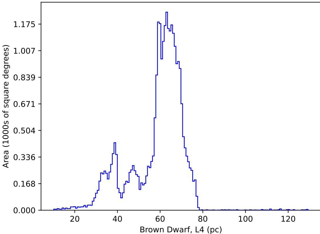
weather_cloudso10v3.4_10yrs : Brown Dwarf, L4
