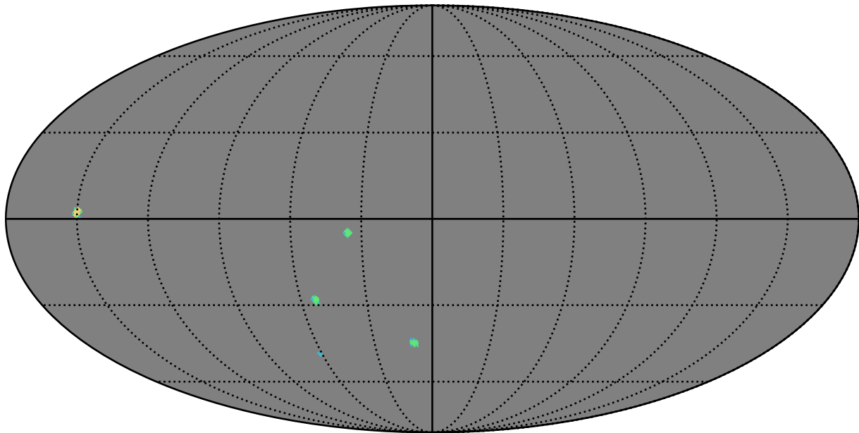
weather_cloudso10v3.4_10yrs z band: AGN_TimeLag_5_days
