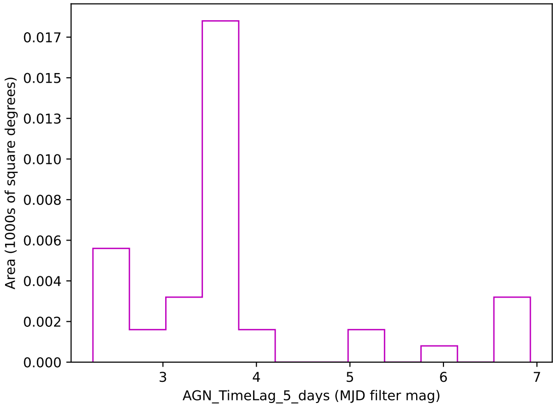
weather_cloudso10v3.4_10yrs z band: AGN_TimeLag_5_days
