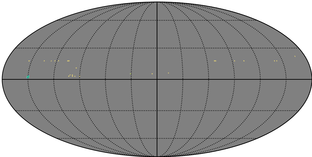
weather_cloudso10v3.4_10yrs y band: AGN_TimeLag_5_days
