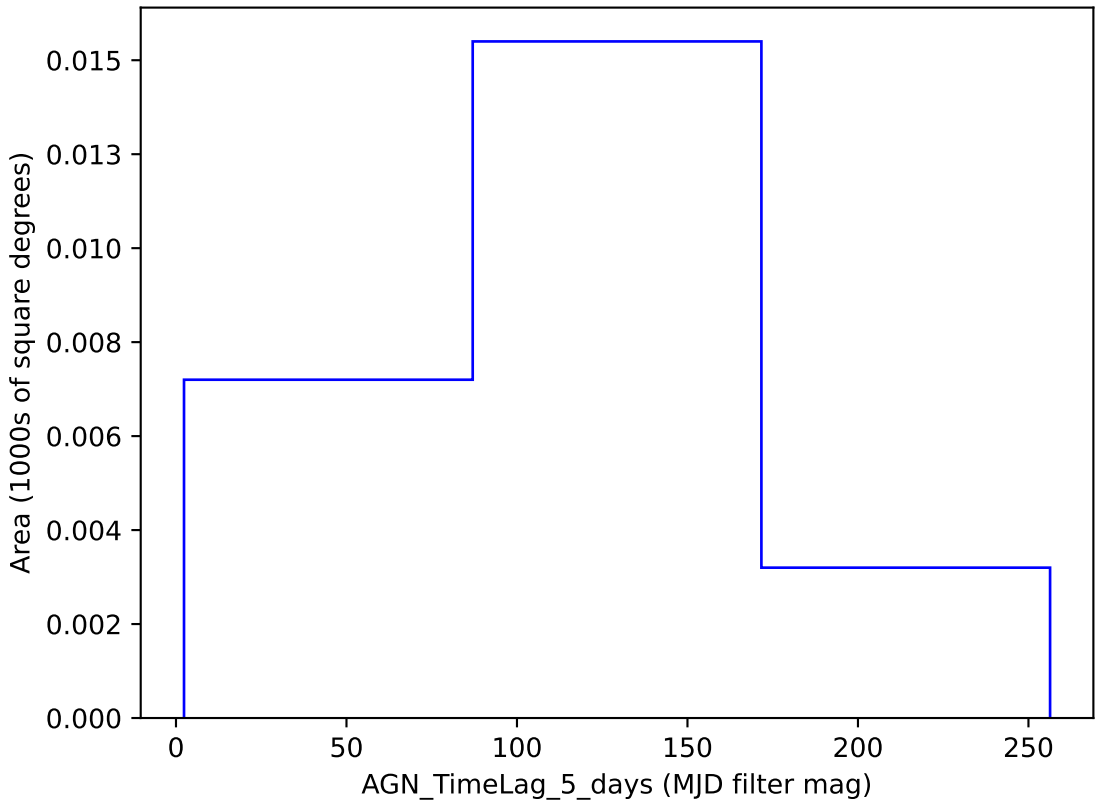
weather_cloudso10v3.4_10yrs y band: AGN_TimeLag_5_days
