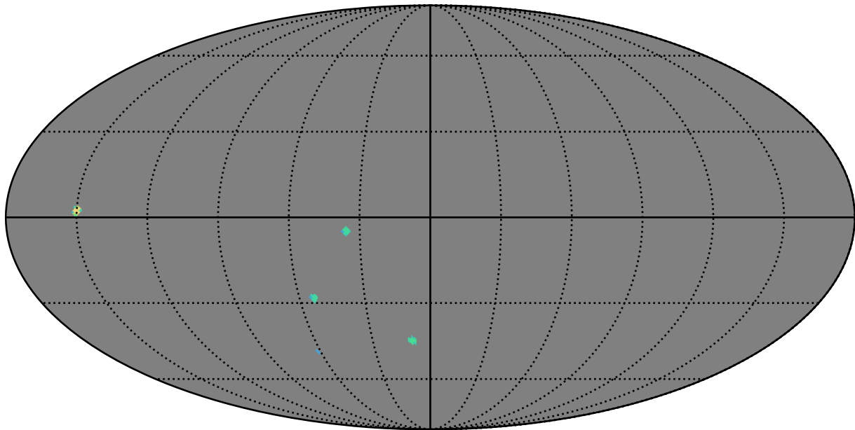
weather_cloudso10v3.4_10yrs r band: AGN_TimeLag_5_days
