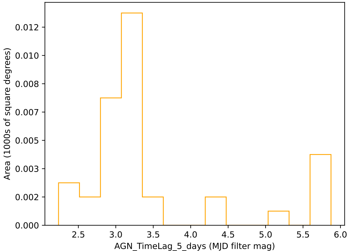
weather_cloudso10v3.4_10yrs r band: AGN_TimeLag_5_days
