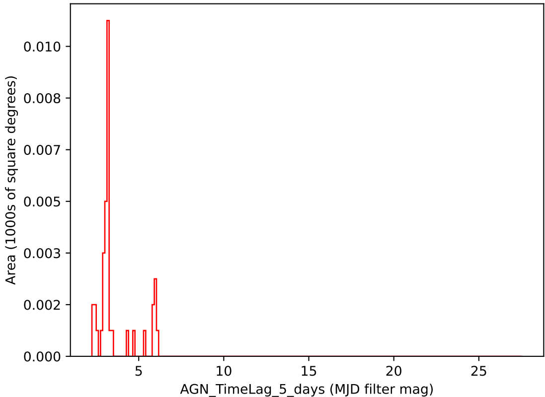
weather_cloudso10v3.4_10yrs i band: AGN_TimeLag_5_days
