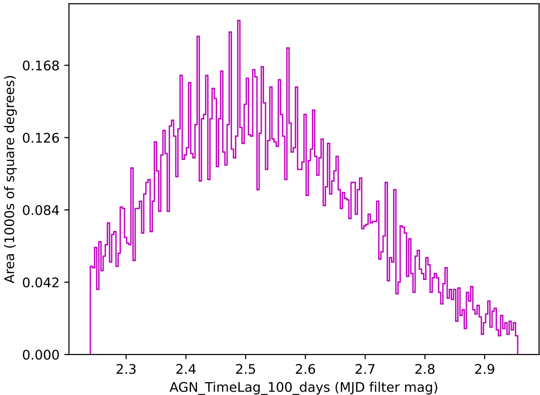
weather_cloudso10v3.4_10yrs z band: AGN_TimeLag_100_days
