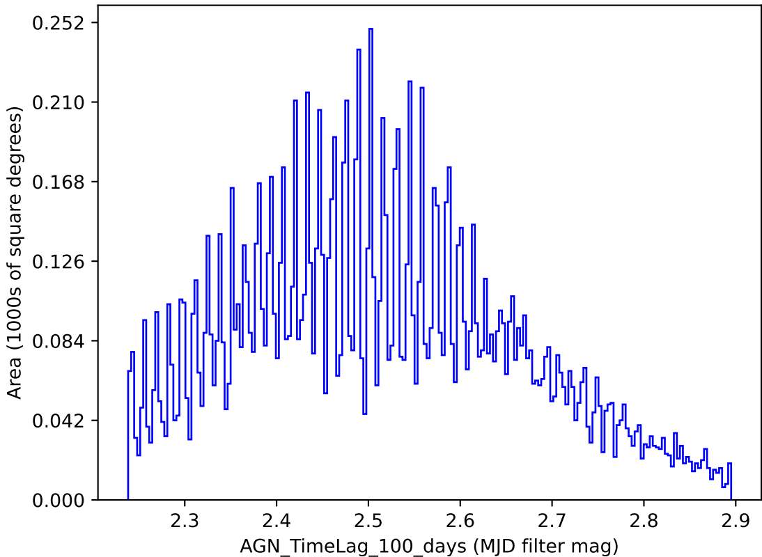
weather_cloudso10v3.4_10yrs y band: AGN_TimeLag_100_days
