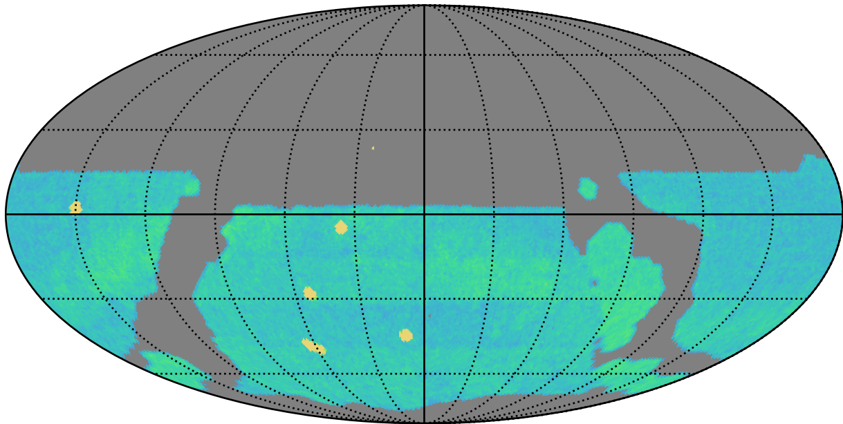
weather_cloudso10v3.4_10yrs r band: AGN_TimeLag_100_days
