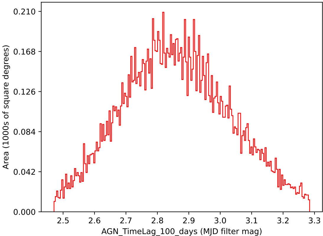
weather_cloudso10v3.4_10yrs i band: AGN_TimeLag_100_days
