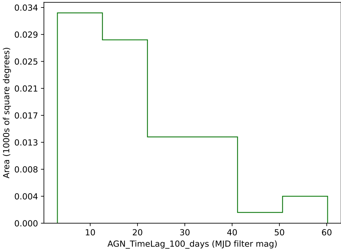
weather_cloudso10v3.4_10yrs g band: AGN_TimeLag_100_days
