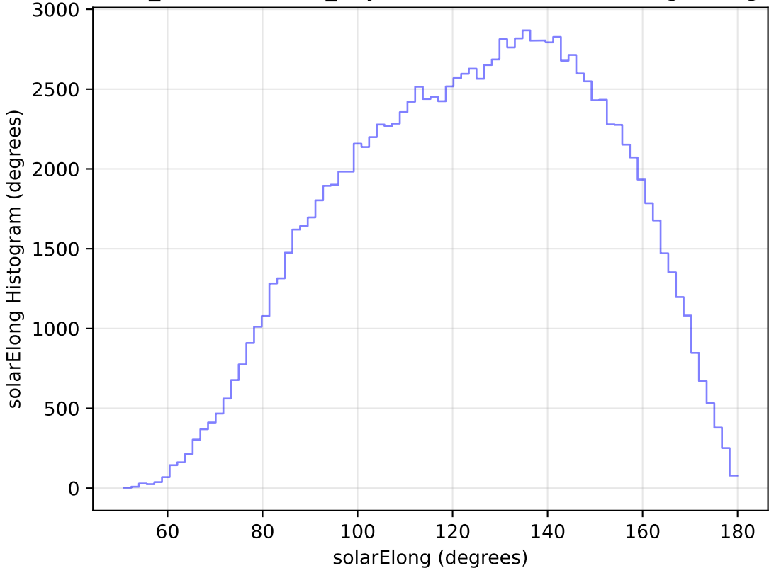
weather_cloudso10v3.4_10yrs WFD u band: solarElong Histogram
