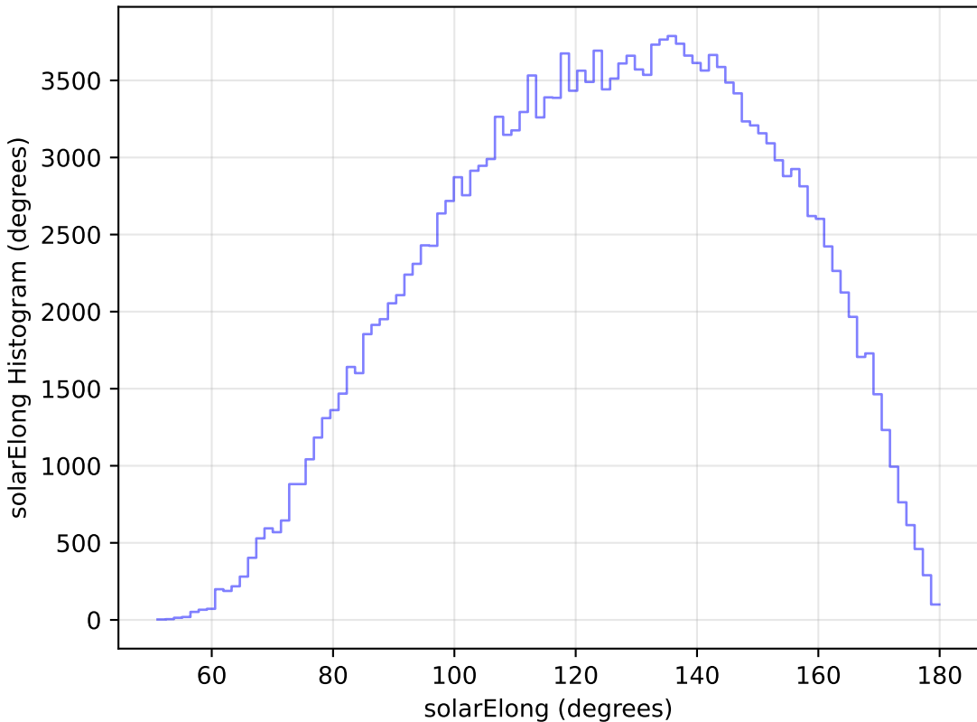
weather_cloudso10v3.4_10yrs WFD g band: solarElong Histogram
