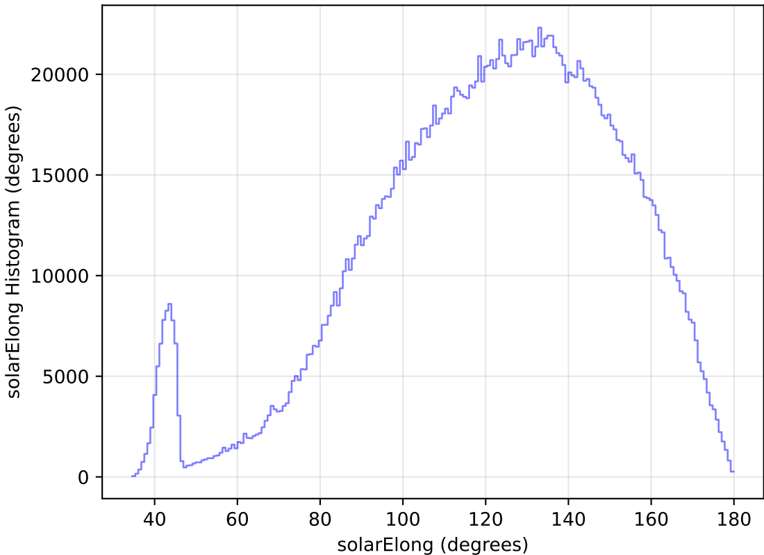
weather_cloudso10v3.4_10yrs WFD all bands: solarElong Histogram
