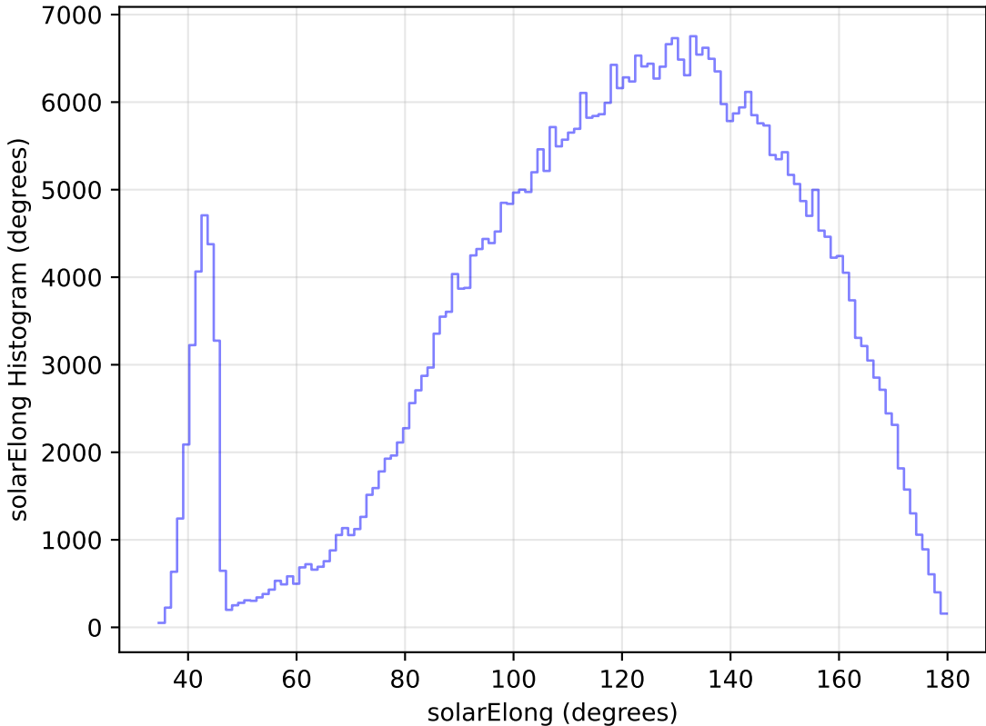
weather_cloudso10v3.4_10yrs All sky z band: solarElong Histogram
