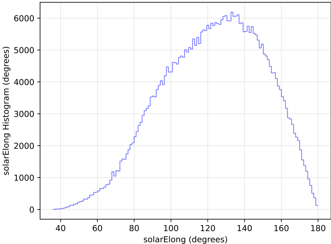
weather_cloudso10v3.4_10yrs All sky y band: solarElong Histogram
