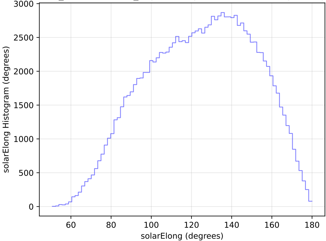
weather_cloudso10v3.4_10yrs All sky u band: solarElong Histogram
