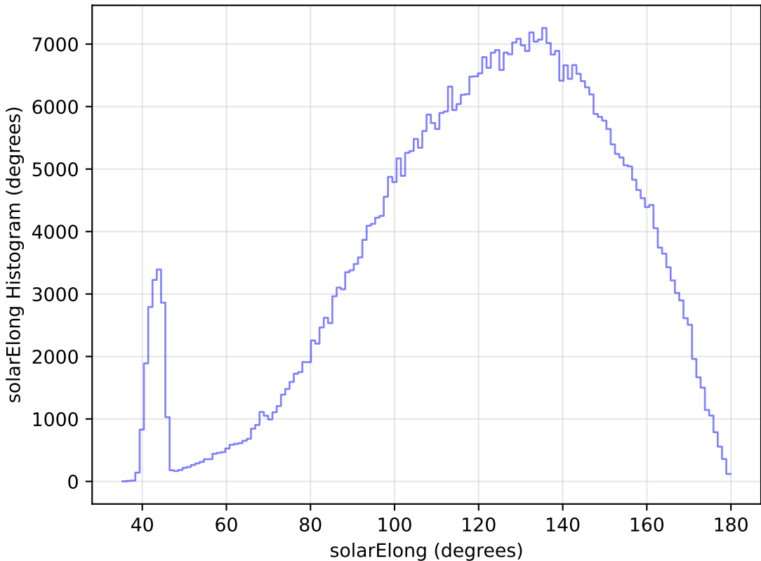
weather_cloudso10v3.4_10yrs All sky r band: solarElong Histogram
