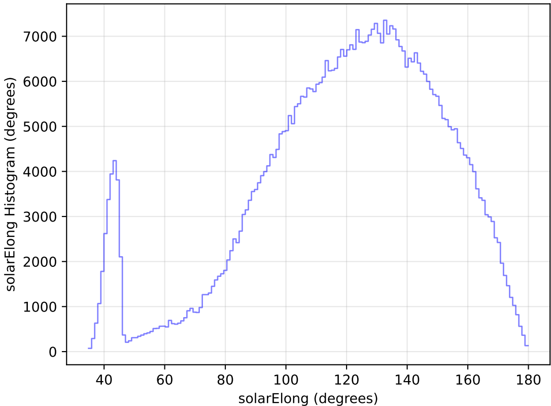
weather_cloudso10v3.4_10yrs All sky i band: solarElong Histogram
