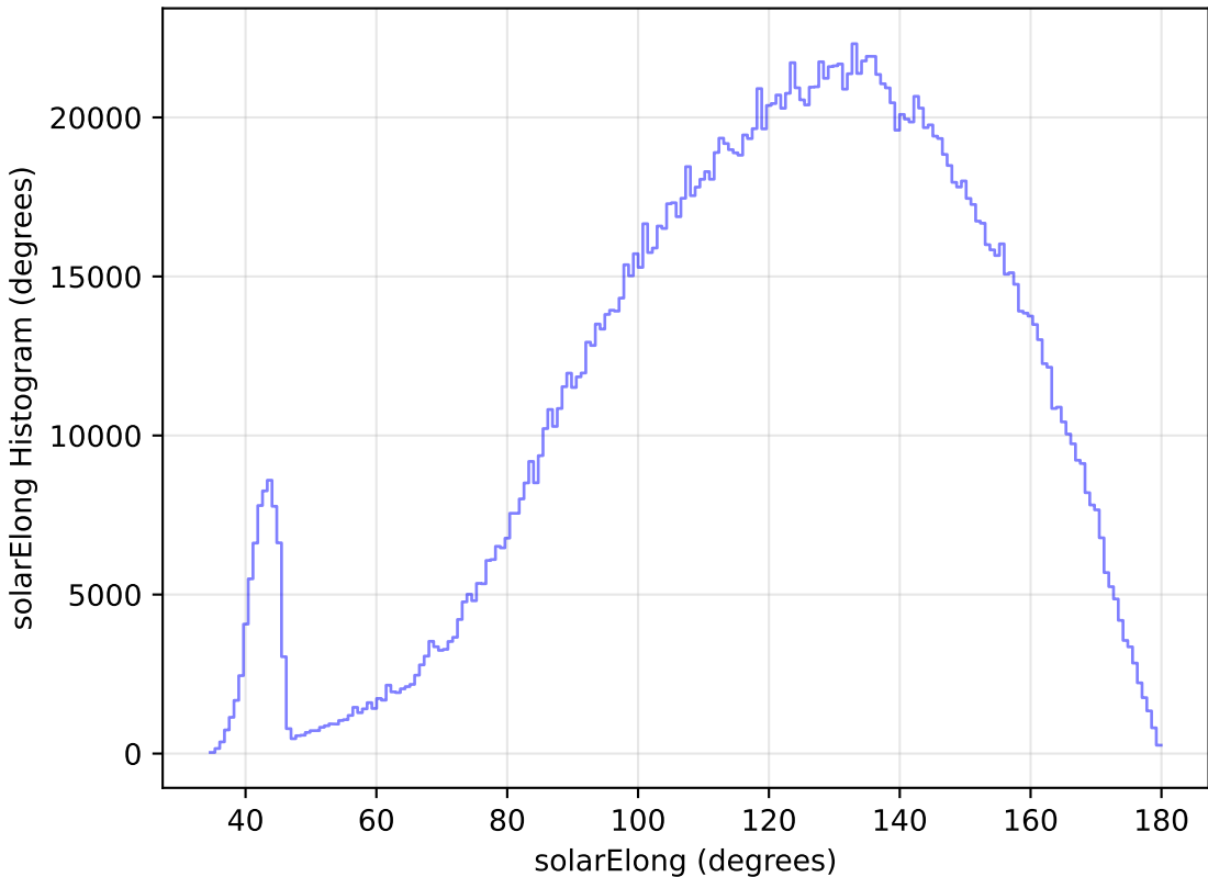
weather_cloudso10v3.4_10yrs All sky all bands: solarElong Histogram
