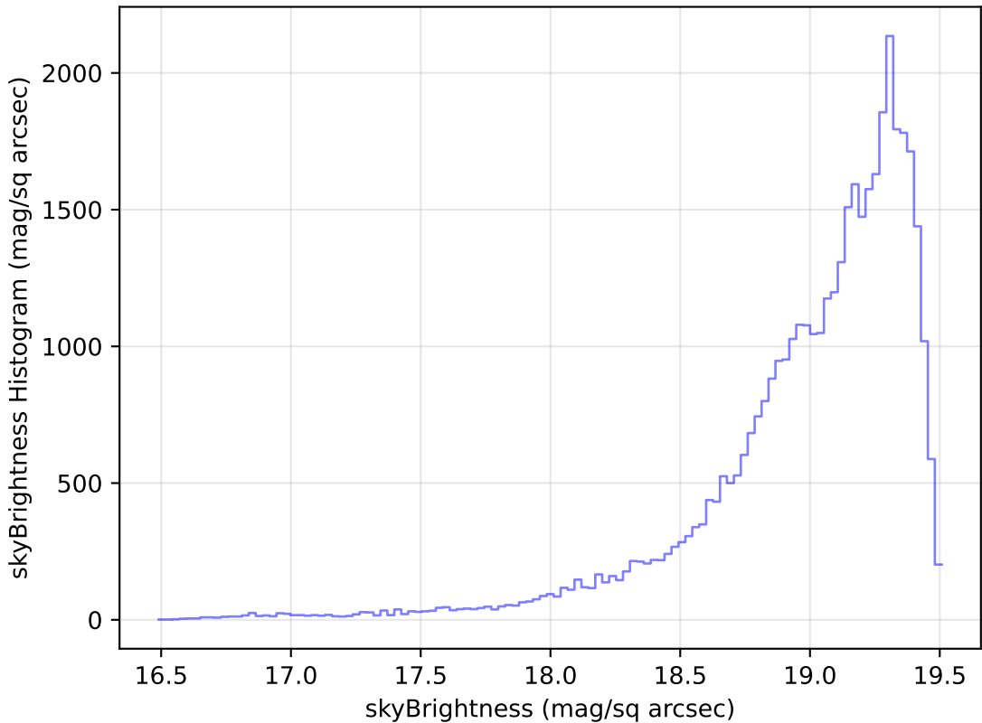
weather_cloudso10v3.4_10yrs Yr 1 z band: skyBrightness Histogram
