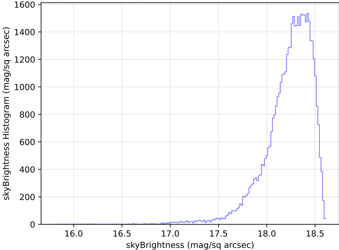
weather_cloudso10v3.4_10yrs Yr 1 y band: skyBrightness Histogram
