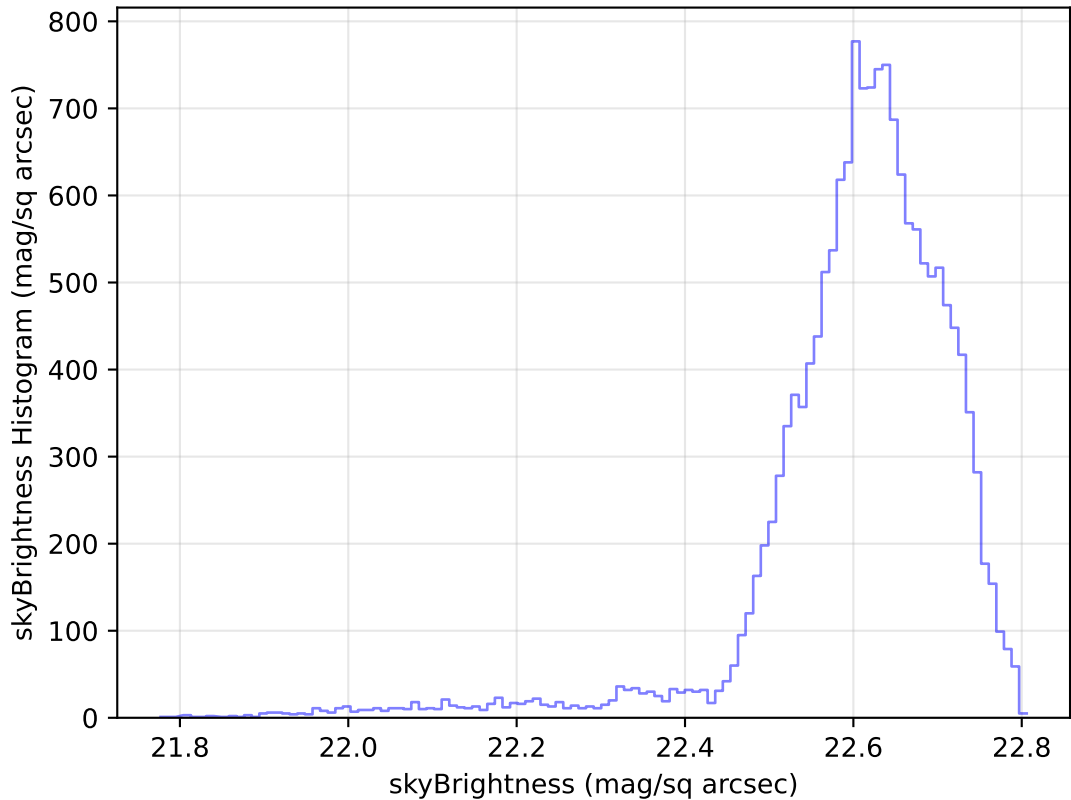
weather_cloudso10v3.4_10yrs Yr 1 u band: skyBrightness Histogram
