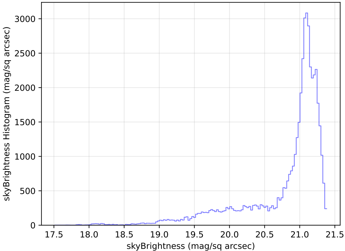
weather_cloudso10v3.4_10yrs Yr 1 r band: skyBrightness Histogram
