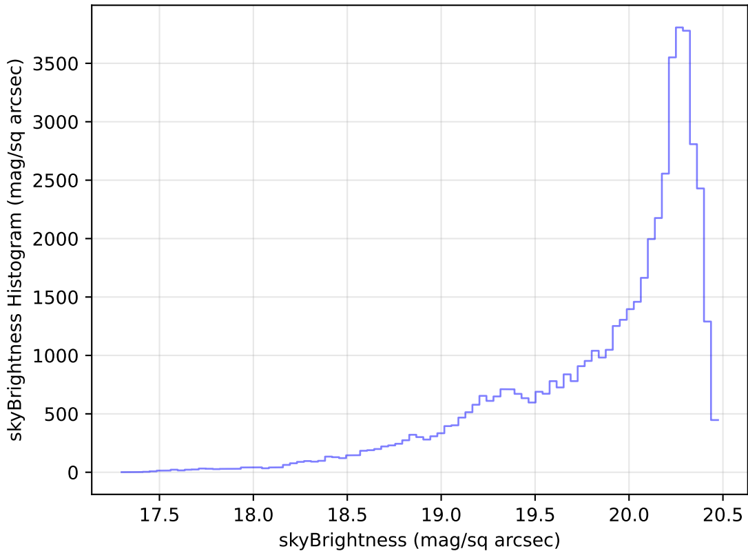
weather_cloudso10v3.4_10yrs Yr 1 i band: skyBrightness Histogram
