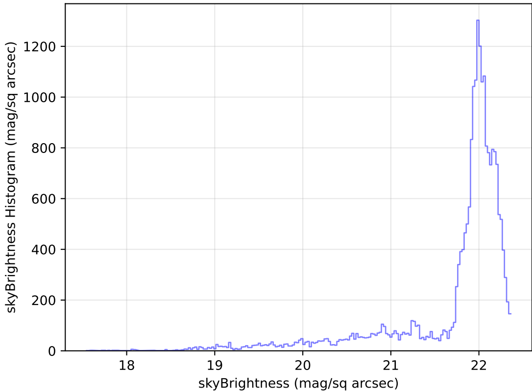
weather_cloudso10v3.4_10yrs Yr 1 g band: skyBrightness Histogram
