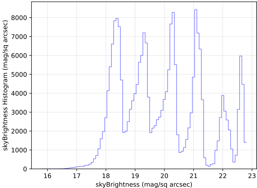
weather_cloudso10v3.4_10yrs Yr 1 all bands: skyBrightness Histogram
