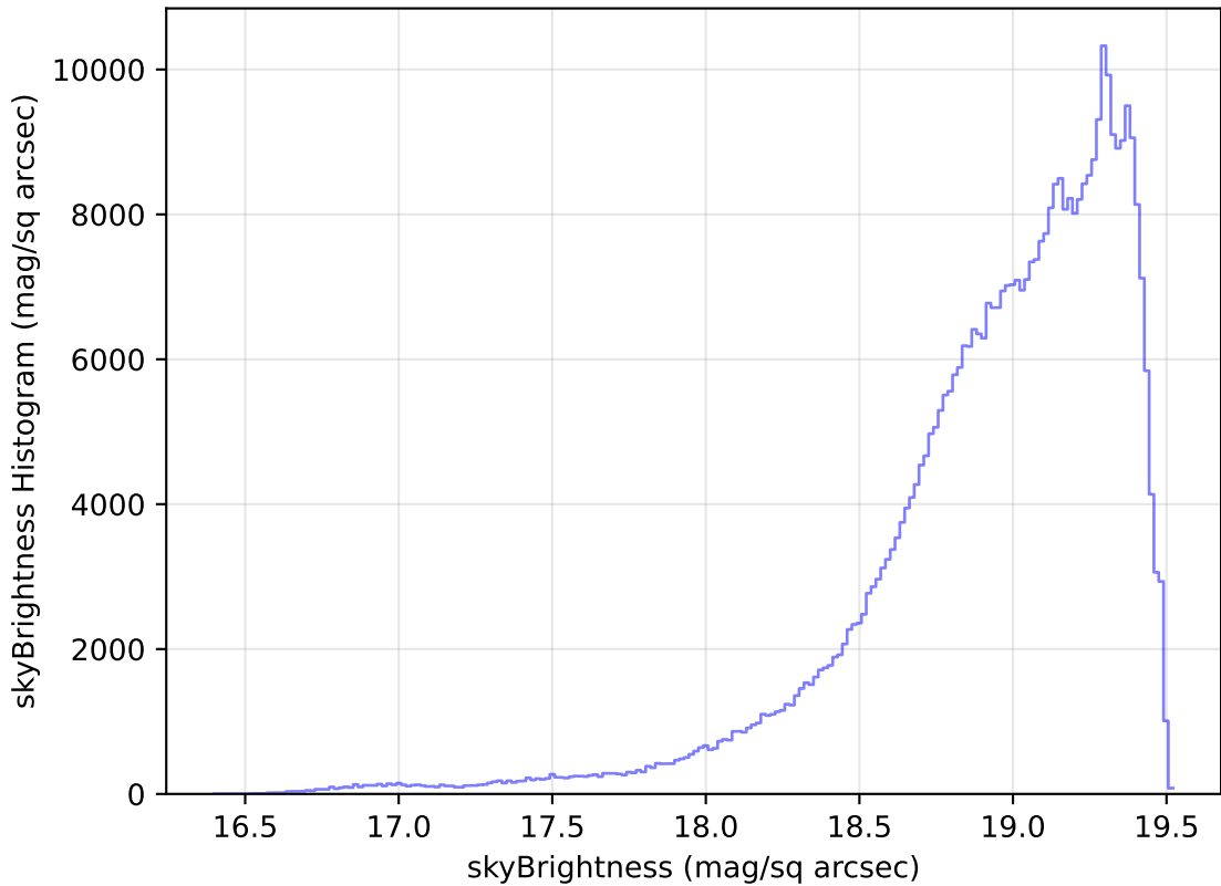
weather_cloudso10v3.4_10yrs WFD z band: skyBrightness Histogram
