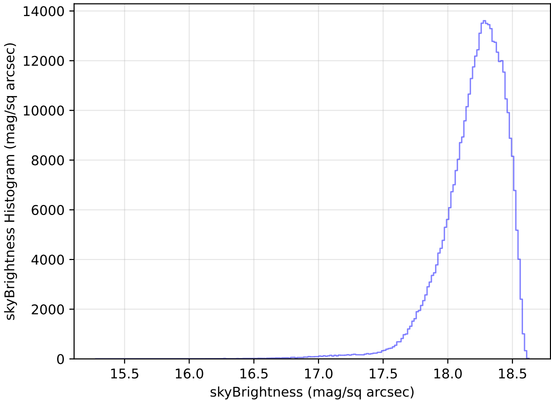
weather_cloudso10v3.4_10yrs WFD y band: skyBrightness Histogram
