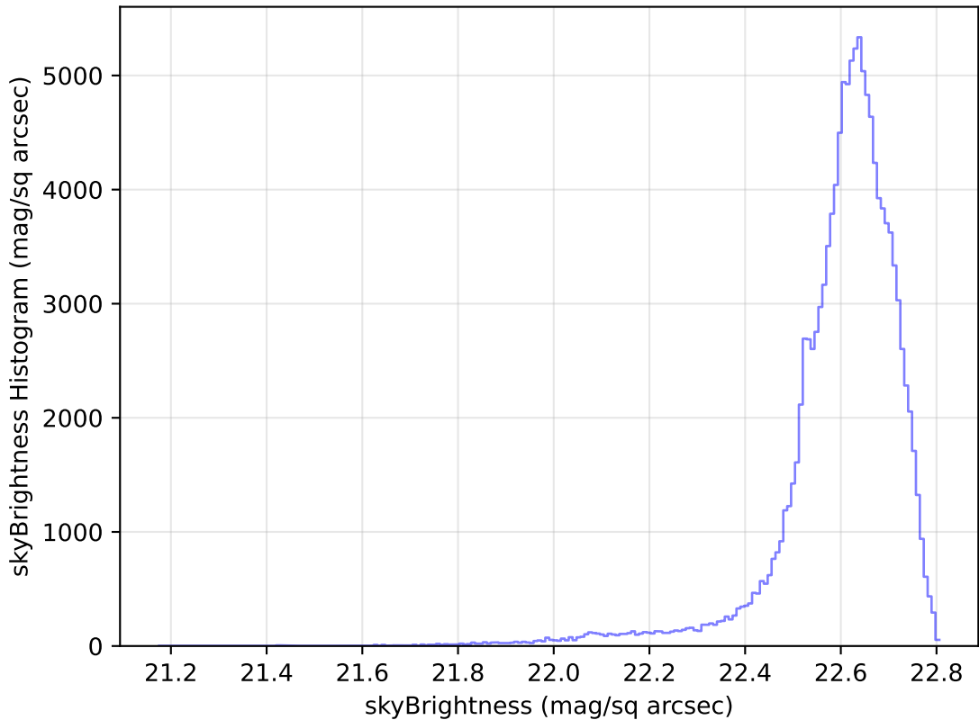
weather_cloudso10v3.4_10yrs WFD u band: skyBrightness Histogram
