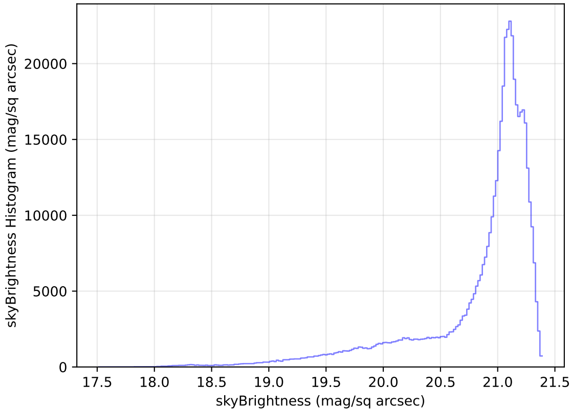
weather_cloudso10v3.4_10yrs WFD r band: skyBrightness Histogram
