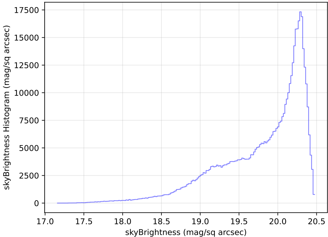
weather_cloudso10v3.4_10yrs WFD i band: skyBrightness Histogram
