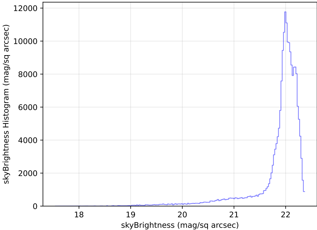
weather_cloudso10v3.4_10yrs WFD g band: skyBrightness Histogram
