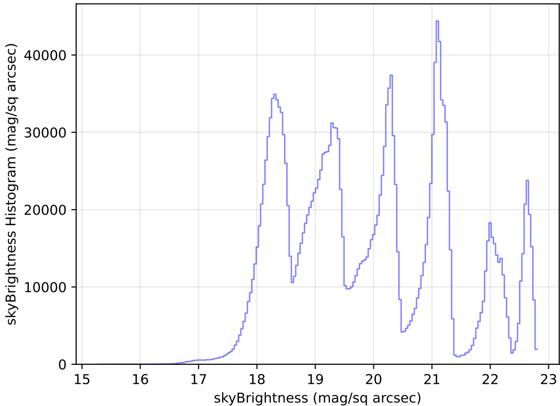
weather_cloudso10v3.4_10yrs WFD all bands: skyBrightness Histogram
