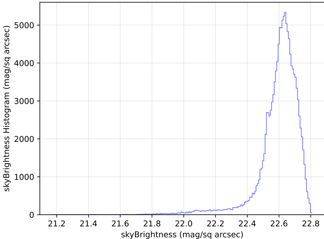
weather_cloudso10v3.4_10yrs All sky u band: skyBrightness Histogram
