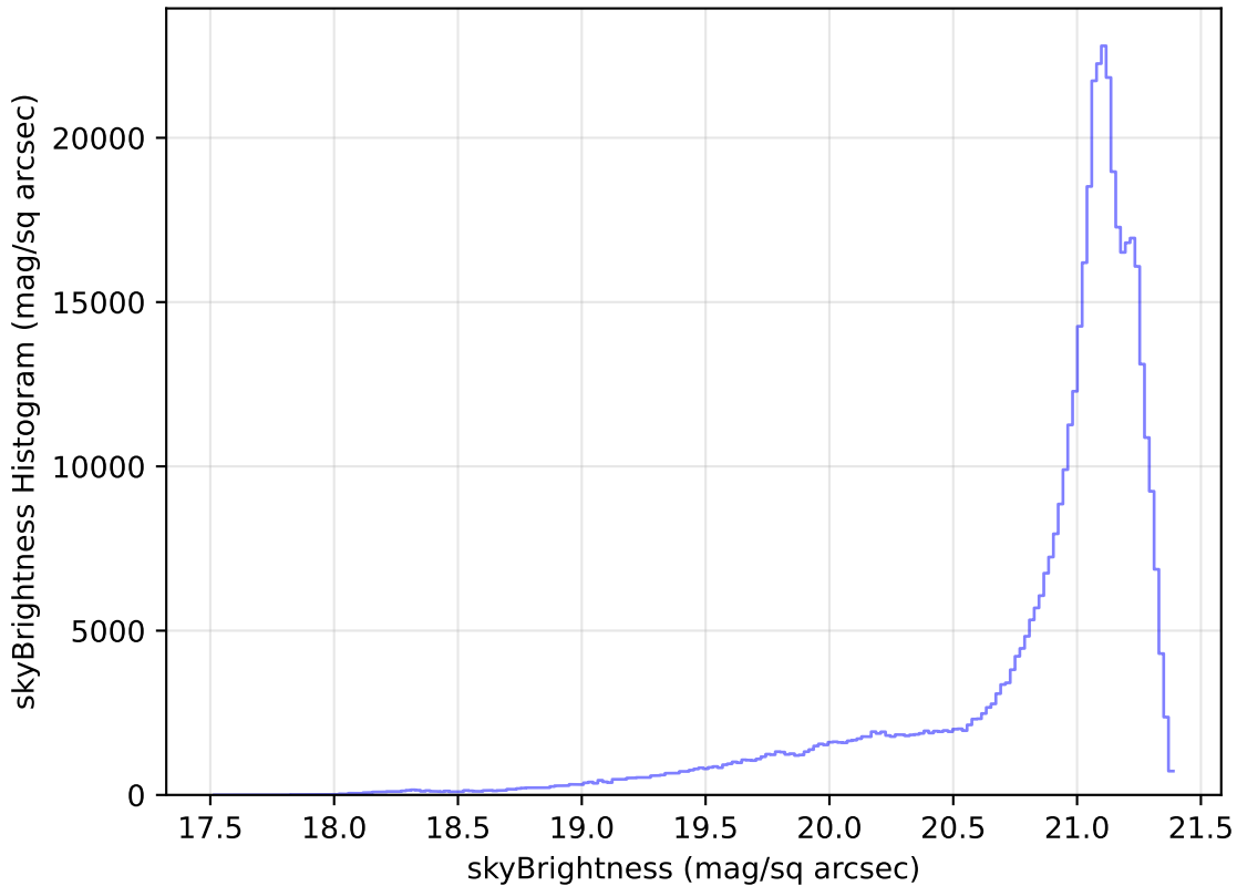
weather_cloudso10v3.4_10yrs All sky r band: skyBrightness Histogram
