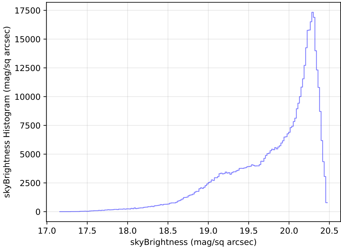
weather_cloudso10v3.4_10yrs All sky i band: skyBrightness Histogram
