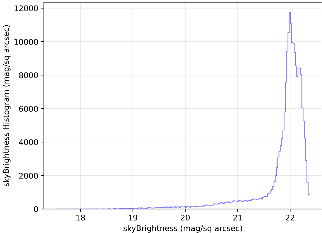
weather_cloudso10v3.4_10yrs All sky g band: skyBrightness Histogram
